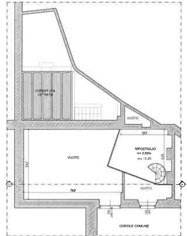
PIANTA PIANO SOPPALCO
